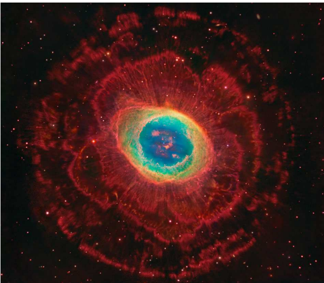
Hubble, Large Binocular Telescope & Subaru Telescope Composition & Copyright: Robert Gendler
